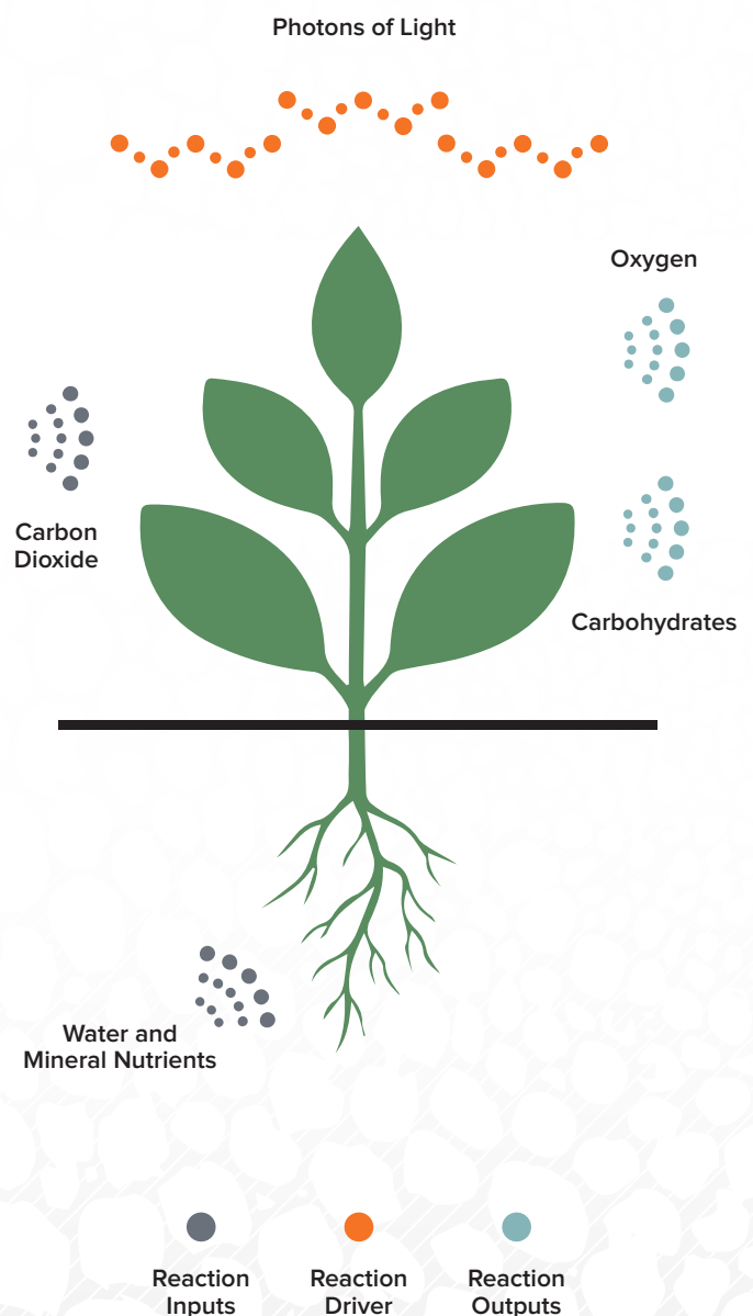
Figure 3: Photosynthesis reaction
