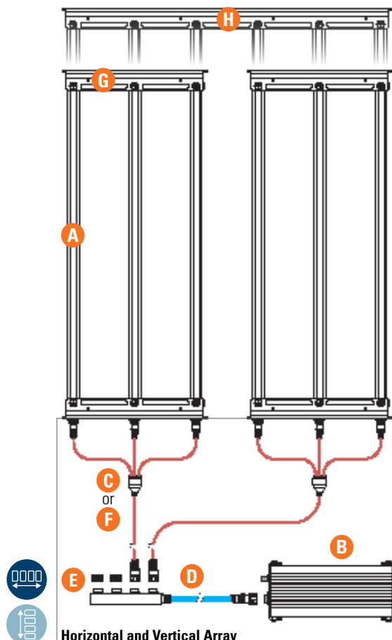
DC CABLE WIRING DIAGRAM
